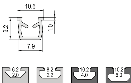
T Slot Reducing Profile-10
