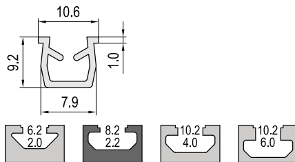
T Slot Reducing Profile-8
